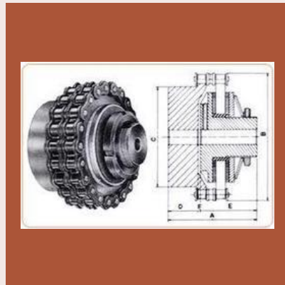
Torque Limiter Couplings
